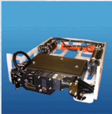
4 FUNCTIONS HYDRAULIC MANIPULATOR
