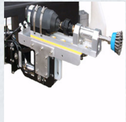
OPTIONAL TOOLS ; VARIOUS CLEANING TOOLS OPTIONS FMD GAMMA RAY, UT GAUGE, LASER ... ETC
